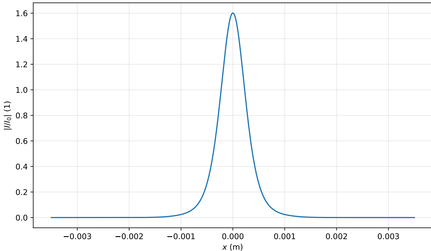
Intensity profile I(x, y = 0, z = 1.672m)/I_0 , P_{in}=0.9P_{cr} , artificial time
